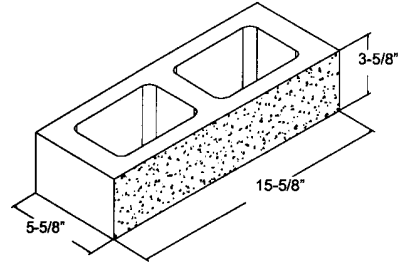
6" x 4" x 16" ** S1S
