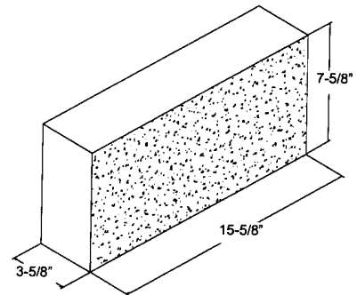
4" x 8" x 16" ** S1S SOLID
