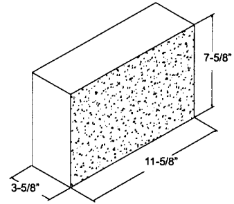
4" x 8" x 12" ** S1S SOLID
