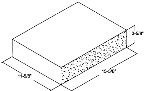
12" x 4" x 16" ** S1S SOLID
