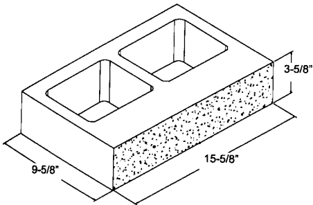
10" x 4" x 16" ** S1S OFFSET CORE
