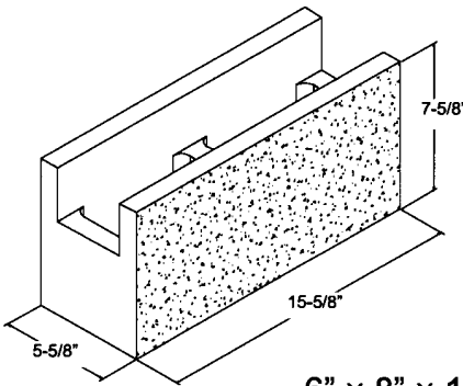
6" x 8" x 16" ** S1S SBBB
