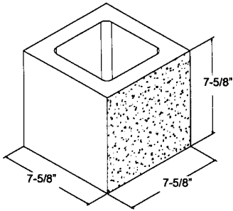
8" x 8" x 8" S1S
