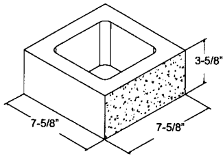
8" x 4" x 8" ** S1S
