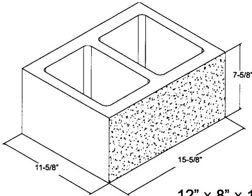
12" x 8" x 16" ** S1S
