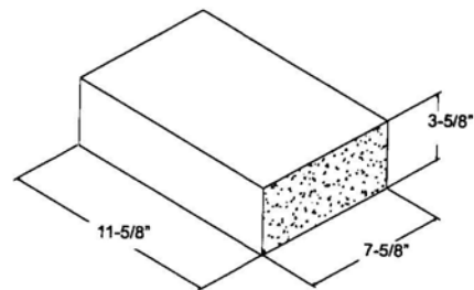
12" x 4" x 8" ** S1S SOLID
