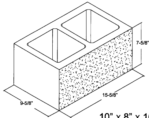
10" x 8" x 16" ** S1S
