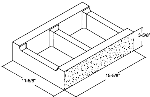
12" x 4" x 16" ** S1S CBB
