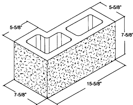
6" x 8" x 16" ** S1S1E RETURN CORNER
