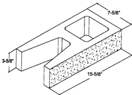
8" x 4" x 16" ** S1S OE1E
