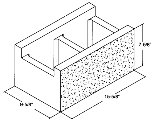
10" x 8" x 16" ** S1S DCBB
