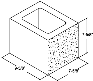
10" x 8" x 8" ** S1S
