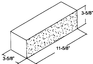
4" x 4" x 12" ** S1S
