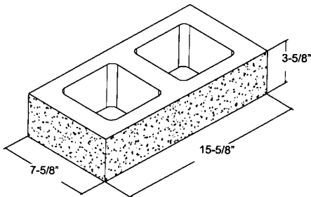
8" x 4" x 16" ** S1S1E
