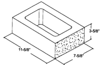
12" x 4" x 8" ** S1S
