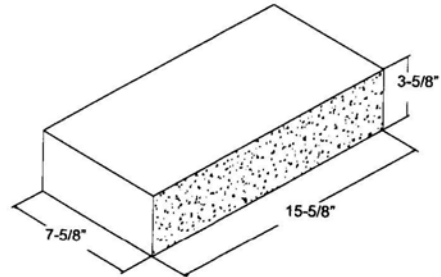
8" x 4" x 16" ** S1S SOLID
