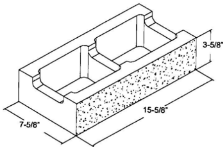
8" x 4" x 16" ** S1S CBB
