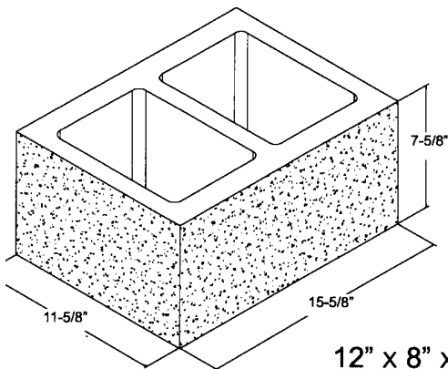
12" x 8" x 16" ** S1S
