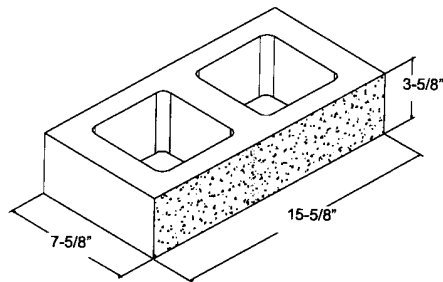
8" x 4" x 16" ** S1S
