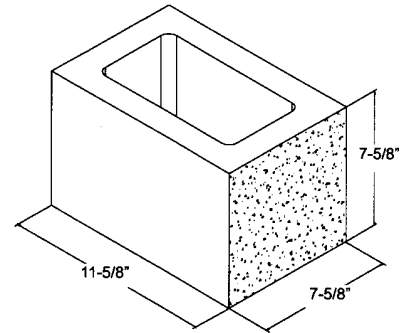
12" x 8" x 8" ** S1S
