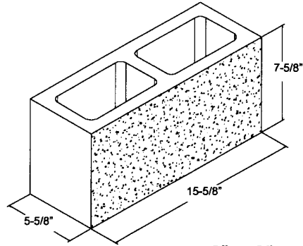
6" x 8" x 16" ** S1S
