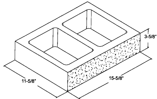
12" x 4" x 16" ** S1S
