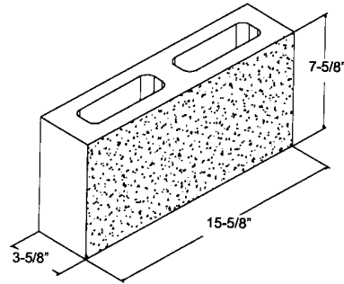
4" x 8" x 16" ** S1S
