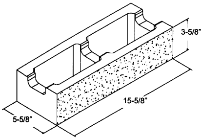
6" x 4" x 16" ** S1S CBB
