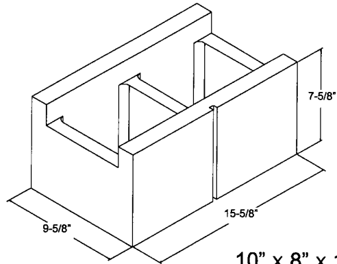
10" x 8" x 16" ** DCBB
