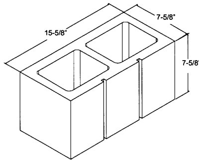
2 SCORE STACKED BOND
