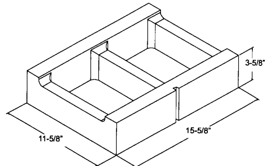
12" x 4" x 16" ** CBB
