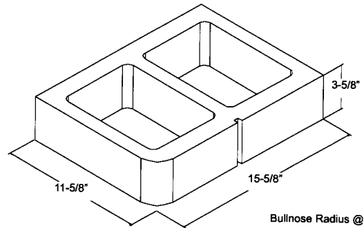
Bullnose Radius @ 2" 12" x 4" x 16" ** SBN AVAILABLE IN DBN & SBNEE
