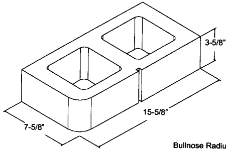
Bullnose Radius @ 2" 8" x 4" x 16" ** SBN AVAILABLE IN DBN & SBNEE
