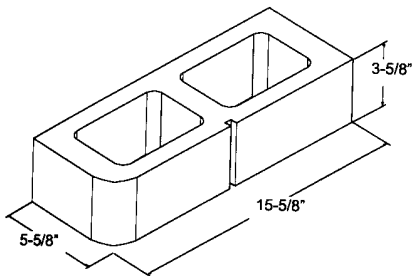
Bullnose Radius @ 2" 6" x 4" x 16" ** SBN AVAILABLE IN DBN & SBNEE
