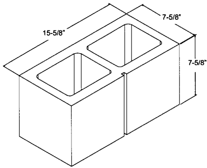
1 SCORE RUNNING OR STACKED BOND
