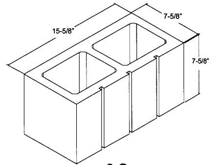
3 SCORE STACKED BOND
