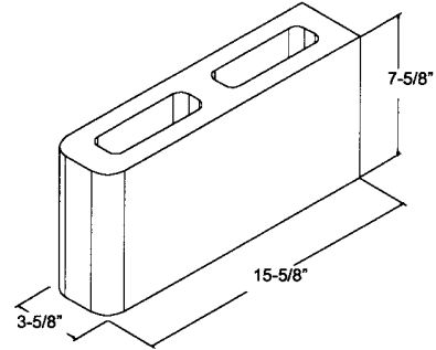
Bullnose Radius @ 2" 4" x 8" x 16" ** DBN
