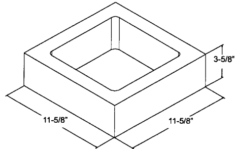
12" x 4" x 12" COLUMN
