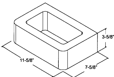
Bullnose Radius @ 2" 12" x 4" x 8" ** DBN
