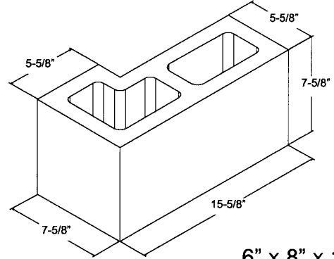
6" x 8" x 16" RETURN CORNER
