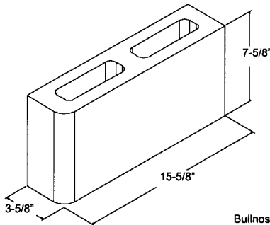
Bullnose Radius @ 2" 4" x 8" x 16" ** SBN
