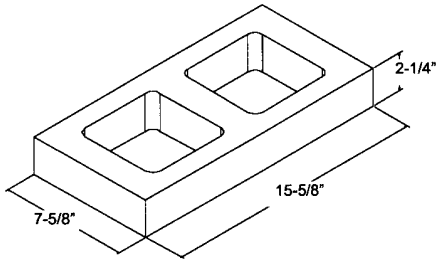
8" x 2" x 16" ** SLIMLINE
