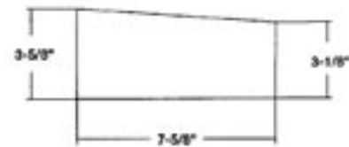
Slope Block Side View
