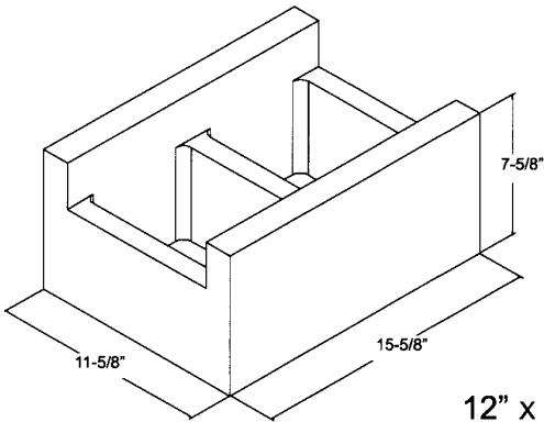
Bullnose Radius @ 2" 12" x 8" x 16" ** SBNEE
