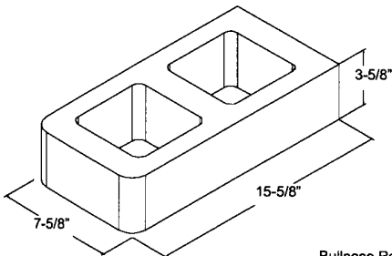
Bullnose Radius @ 2" 8" x 4" x 16" ** DBN
