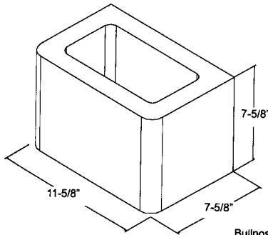
Bullnose Radius @ 2" 12" x 8" x 8" ** DBN
