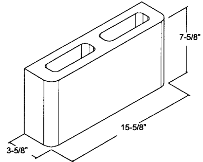
Bullnose Radius @ 2" 4" x 8" x 16" ** SBNEE
