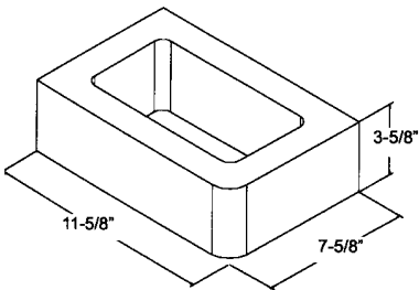
Bullnose Radius @ 2" 12" x 4" x 8" ** SBN
