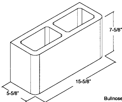
Bullnose Radius @ 2" 6" x 8" x 16" ** SBNEE
