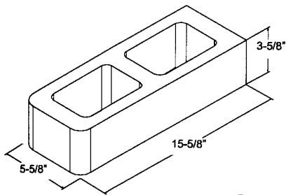
Bullnose Radius @ 2" 6" x 4" x 16" ** DBN
