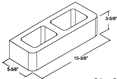
Bullnose Radius @ 2" 6" x 4" x 16" ** SBNEE
