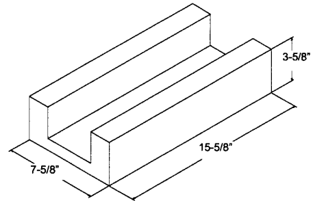
8" x 4" x 16" LINTEL
