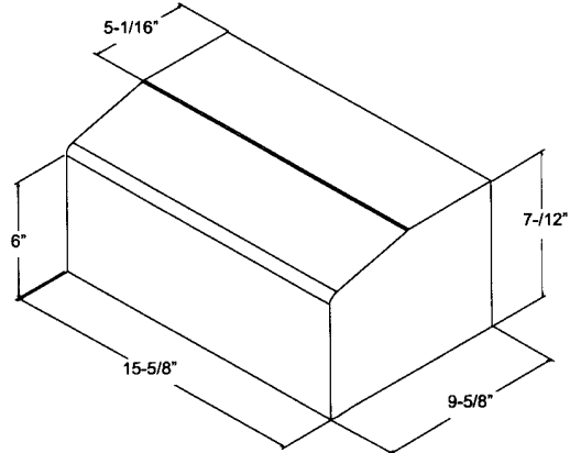
10" x 8" x 16" ** SILL BLOCK
