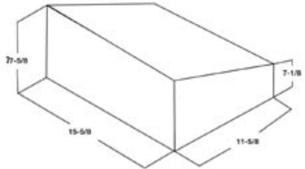
12" x 8" x 16" ** SLOPE BLOCK
