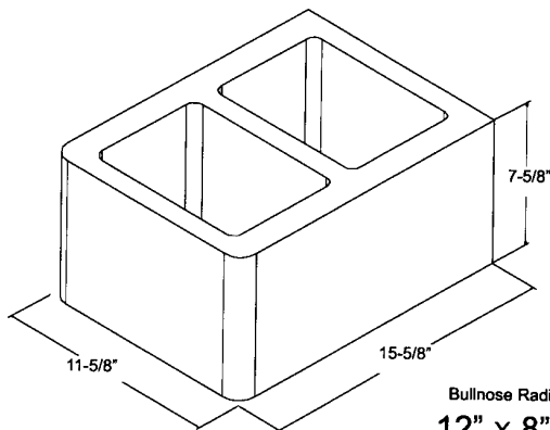
Bullnose Radius @ 2" 12" x 8" x 16" ** SBN
