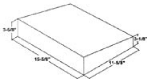
12" x 4" x 16" ** SLOPE BLOCK
