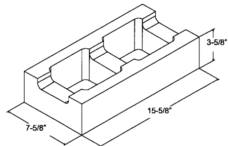
8" x 4" x 16" CBB
