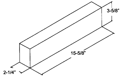
2-1/4" x 4" x 16" ROMAN
