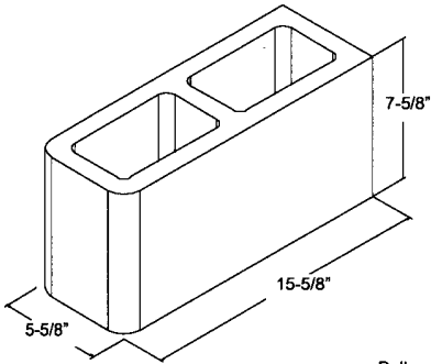
Bullnose Radius @ 2" 6" x 8" x 16" ** DBN
