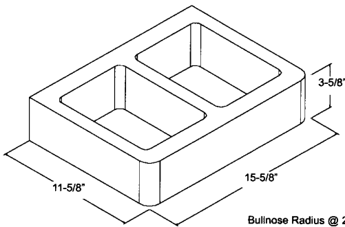
Bullnose Radius @ 2" 12" x 4" x 16" ** SBNEE
