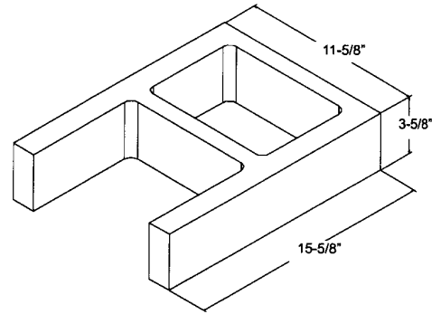
12" x 4" x 16" ** OE1E
