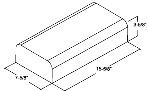
8" x 4" x 16" ** ROUND TOP
