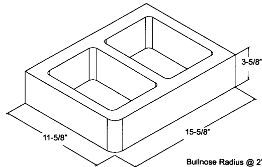
Bullnose Radius @ 2" 12" x 4" x 16" ** SBN
