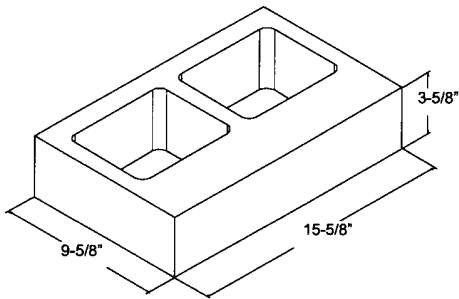
10" x 4" x 16" ** OFFSET CORE
