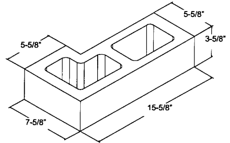
6" x 4" x 16" RETURN CORNER
