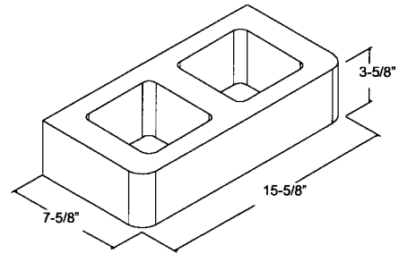
Bullnose Radius @ 2" 8" x 4" x 16" ** SBNEE
