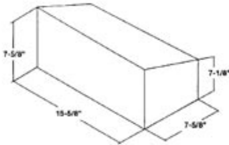
8" x 8" x 16" ** SLOPE BLOCK
