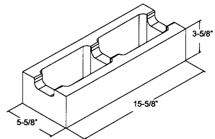
6" x 4" x 16" CBB
