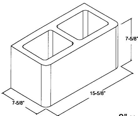
8" x 8" x 16" SBNEE
