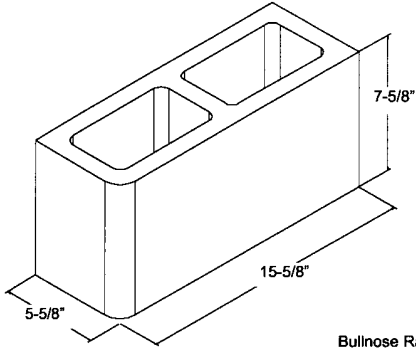
Bullnose Radius @ 2" 6" x 8" x 16" ** SBN
