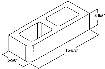
Bullnose Radius @ 2" 6" x 4" x 16" ** SBN
