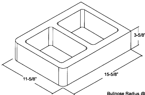
Bullnose Radius @ 2" 12" x 4" x 16" ** DBN
