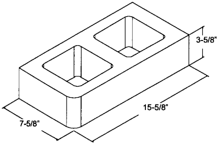
Bullnose Radius @ 2" 8" x 4" x 16" ** SBN
