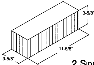
2 SIDES 2 SIDES 1 END 4" X 4" X 12" ** SOLID
