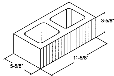
2 SIDES 6" X 4" X 12" **
