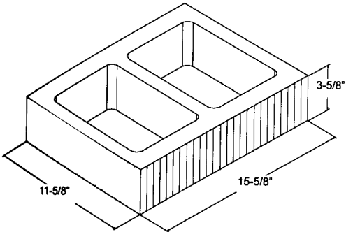
2 SIDES 12" x 4" x 16" **
